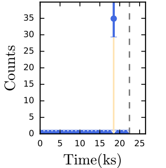
XRT 191127; T_{90} = 0.3_{-0.2}^{+0.2} ks
