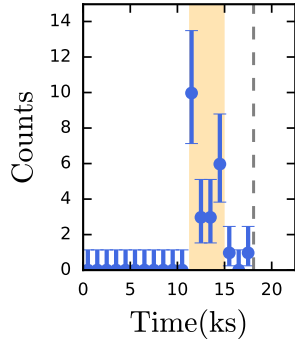
XRT 191223; T_{90} = 3.7_{-0.5}^{+2.4} ks
