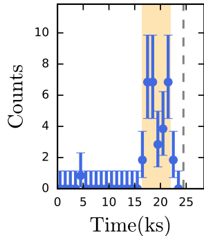
XRT 191223; T_{90} = 3.7_{-0.5}^{+2.4} ks
