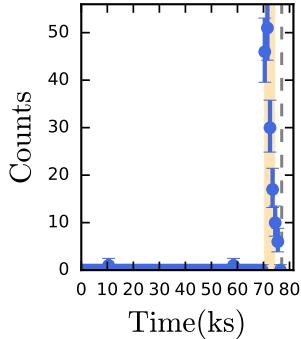
XRT 170901; T_{90} = 3.9_{-0.7}^{+1.2} ks
