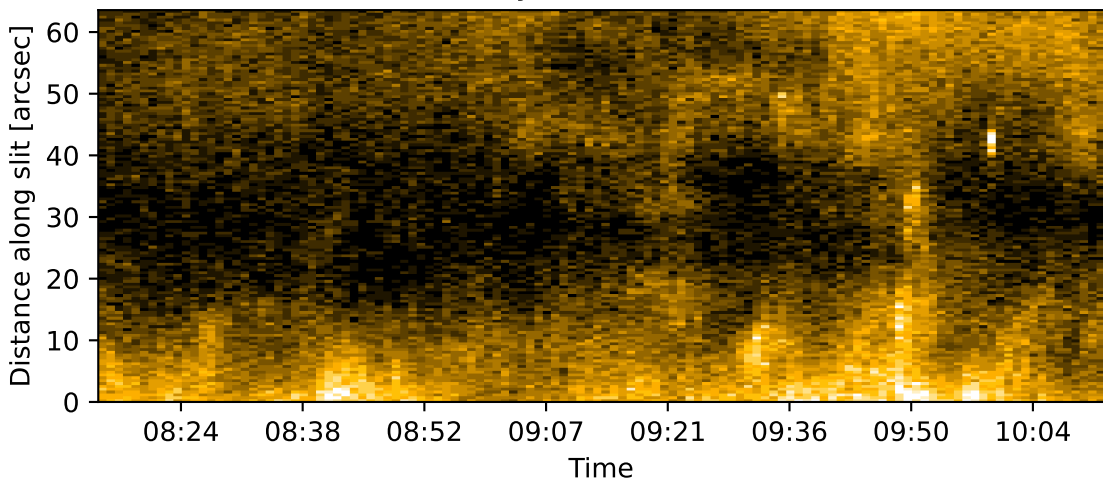
Intensity in 174 Å EUV/HRI
