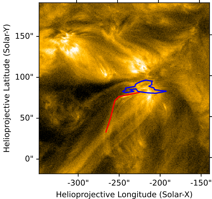
HRI 174 Å image at 09:49:15
