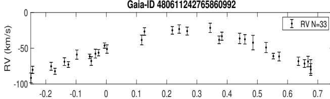
Gaia-ID 480611242765860992
