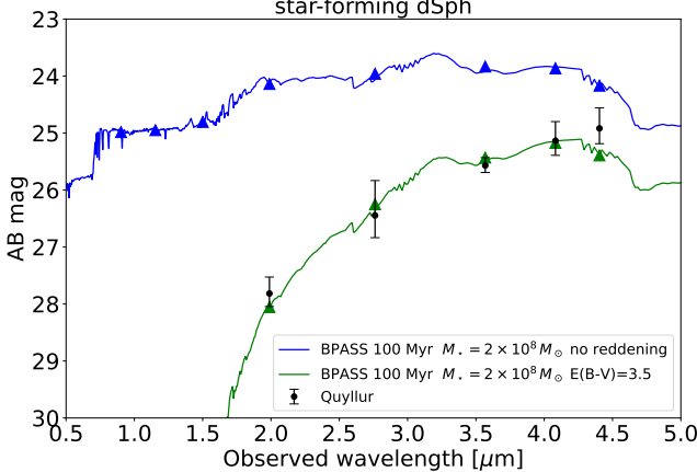
star-forming dSph
