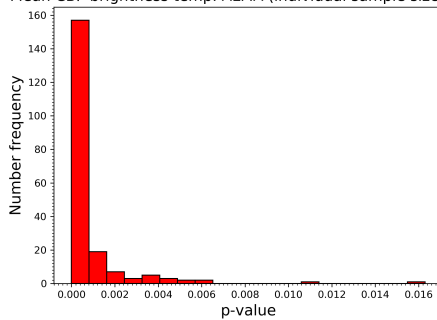
Mean CBP brightness temp. ALMA (individual sample size = 18)
