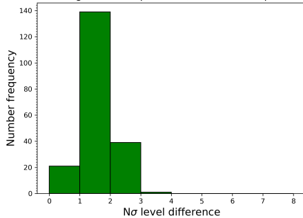
Mean CBP brightness temp. ALMA (individual sample size = 16)
