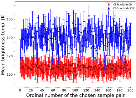
Mean CBP brightness temp. ALMA (individual sample size = 16)
