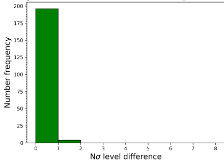
Projected CBP area SDO/AIA (individual sample size = 30)
