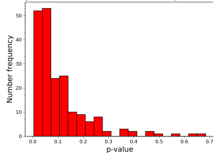
Projected CBP area SDO/AIA (individual sample size = 16)
