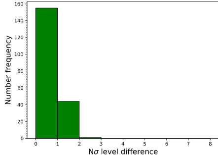
Projected CBP area SDO/AIA (individual sample size = 5)
