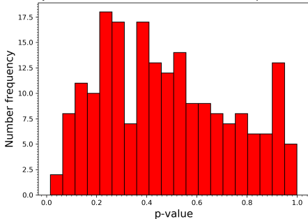
Projected CBP area SDO/AIA (individual sample size = 5)
