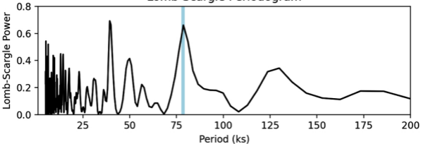
Lomb-Scargle Periodogram
