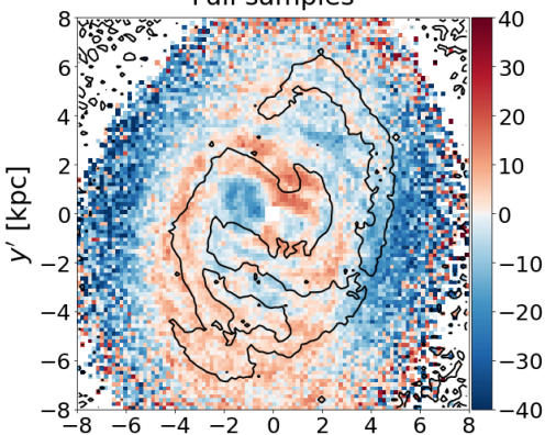
Full samples
