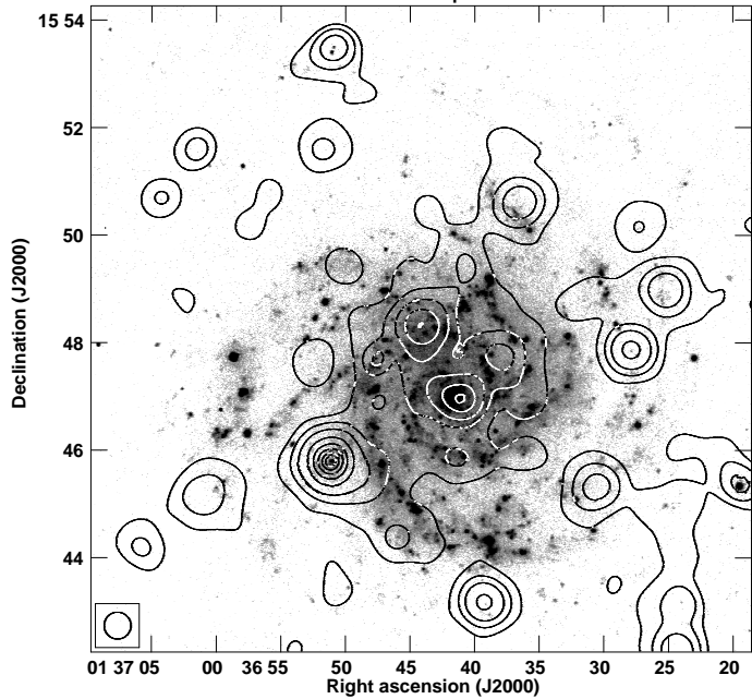
NGC628 XMM-Newton EPIC 1-2 keV on Optical Monitor UVW1
