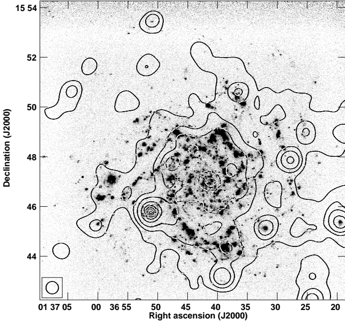
NGC628 XMM-Newton EPIC 0.2-1 keV on Halpha
