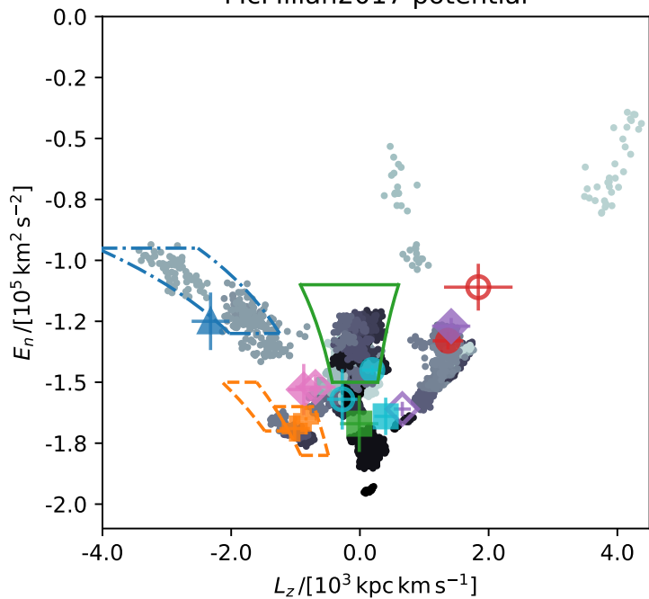
McMillan2017 potential
