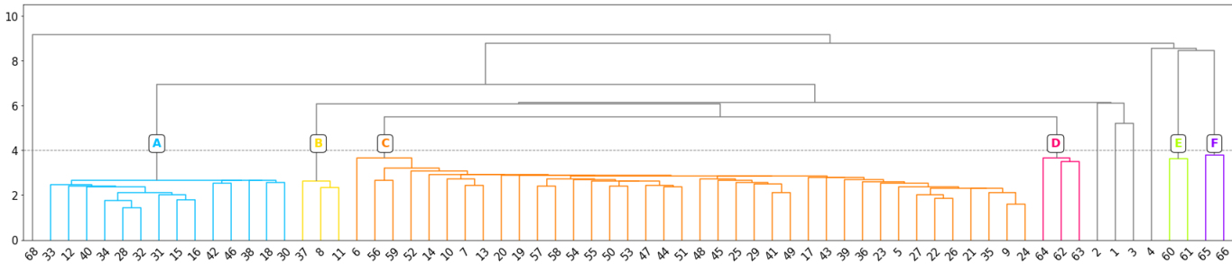
Mahalanobis distance
