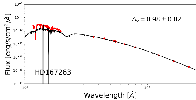
(x) HD 167263
