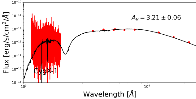
(a) Cyg X-1
