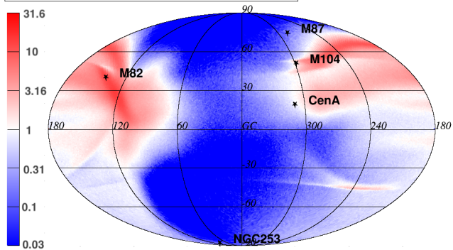
Magnification Factor: p @ \text{Log}(E/[eV]) = 18.6
