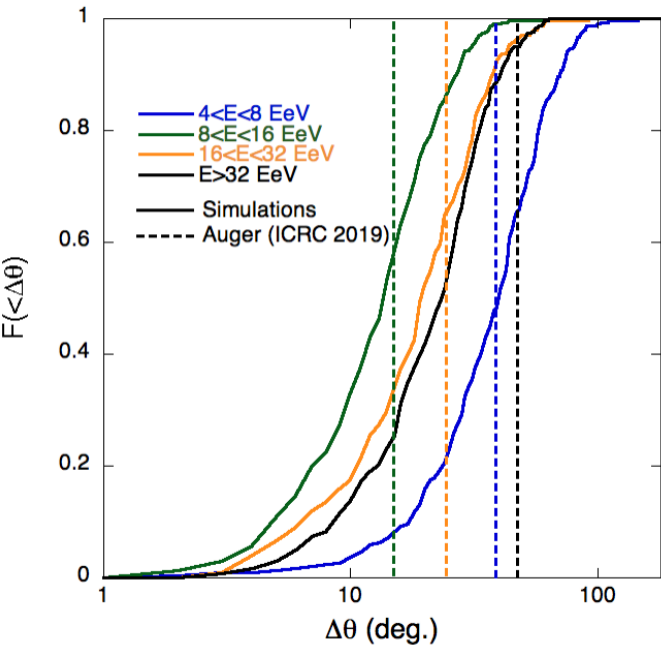
Dipole angular separation w.r.t the E > 8 EeV energy bin
