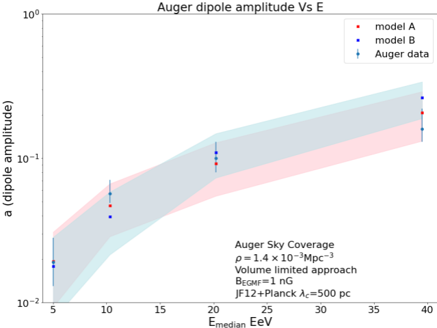
Auger dipole amplitude Vs E
