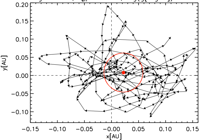
st36gm00n05, T_{\text{eff}}=3710 K, \log(g[\text{c.g.s.}])=0.047
