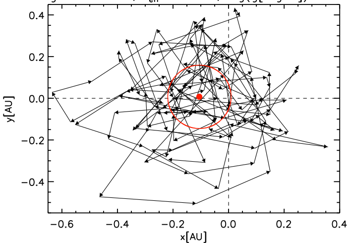
st36gm00n04, T_{\text{eff}}=3663 K, \log(g[\text{c.g.s.}])=0.023
