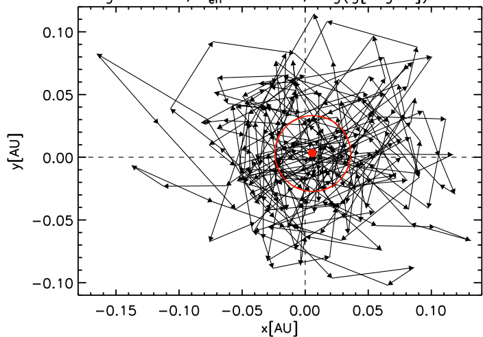
st36g00n06, T_{\text{eff}}=3660 K, \log(g[\text{c.g.s.}])=0.009
