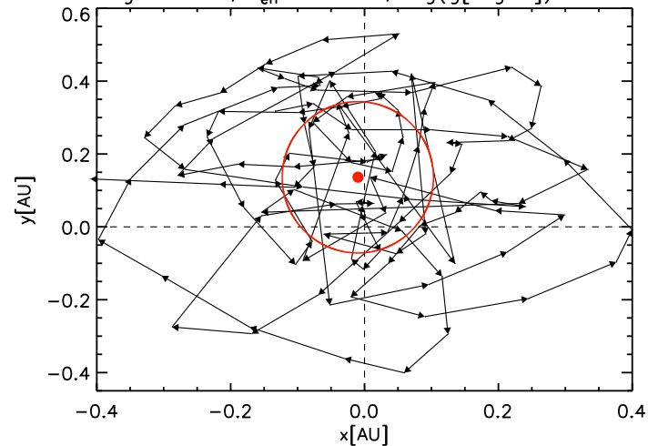
st35gm03n13, T_{\text{eff}}=3430 K, \log(g[\text{c.g.s.}])=-0.354
