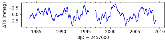
\iota Her (s025)
