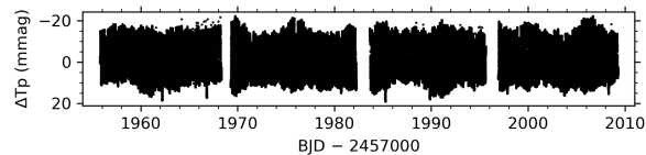
\beta Cep (s024+s025)
