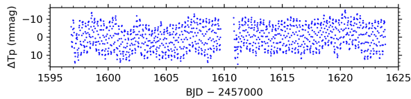
\alpha Lup (s011)
