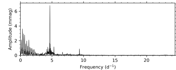
\kappa Sco (s039)
