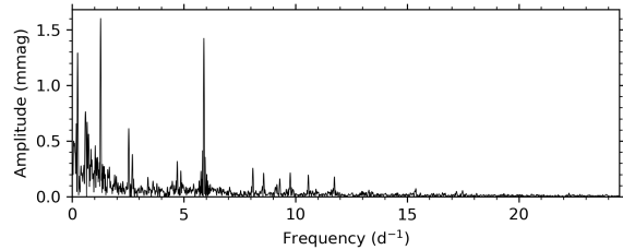
\lambda Sco (s039)
