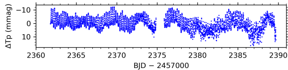
\kappa Sco (s039)
