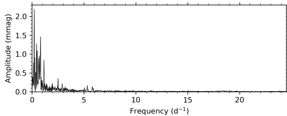
\iota Her (s025)
