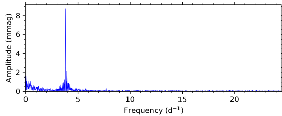
\epsilon Lup (s038)
