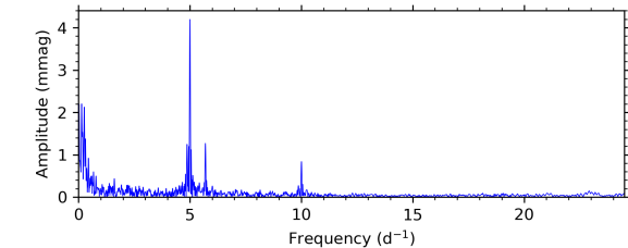
\beta Cep (s024+s025)
