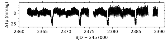
\lambda Sco (s039)
