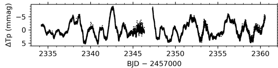
\epsilon Lup (s038)
