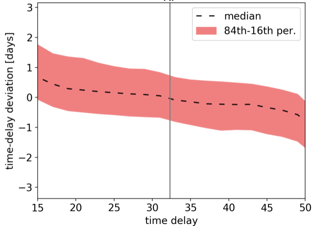
RF
