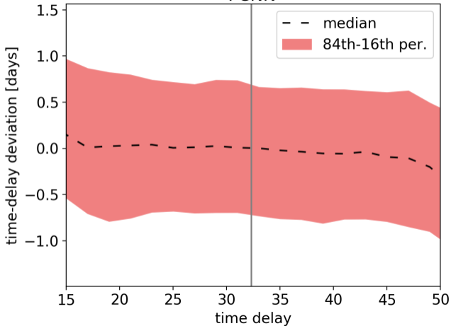
FCNN
