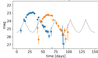
W7 model, r band, z_s = 0.76
