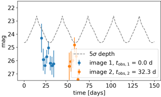
W7 model, u band, z_s = 0.76
