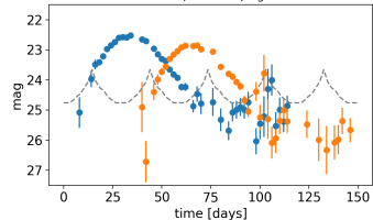
W7 model, i band, z_s = 0.76
