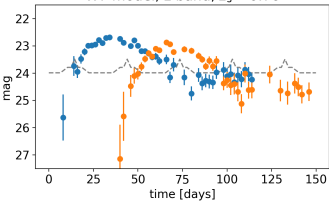
W7 model, z band, z_s = 0.76
