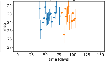
W7 model, H band, z_s = 0.76
