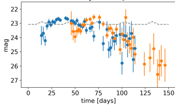
W7 model, y band, z_s = 0.76
