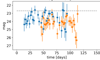
W7 model, J band, z_s = 0.76
