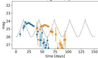
W7 model, g band, z_s = 0.76
