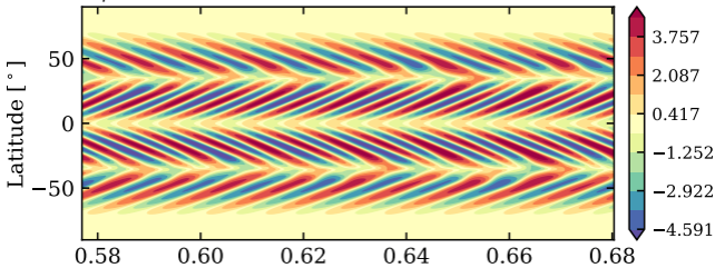
B_r/B_0 ( 10^{-4} ) at r = 1.0 R_\odot
