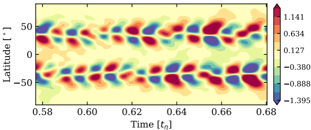
B_r/B_0 ( 10^{-4} ) at r = 1.0 R_\odot
