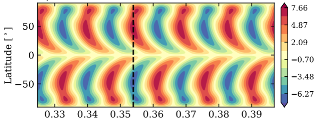
B_r/B_0 at r = 1.0 R_\odot
