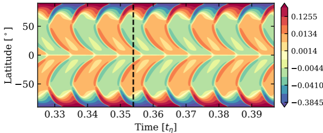
B_r/B_0 at r = 1.0 R_\odot
