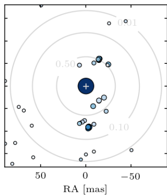
S38-pointings
