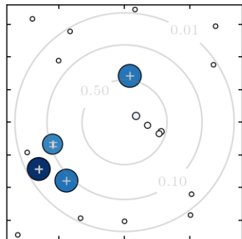
mid-pointings
