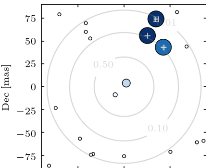
SE-pointings
