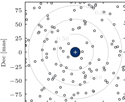
SE-pointings
