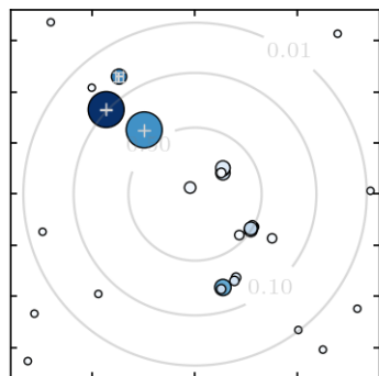
S38-pointings
