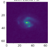
With Euclid PSF
