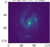
Original HST image
