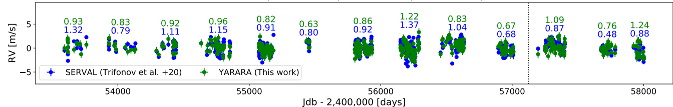
SERVAL (rms : 1.13 m/s) vs YARARA (rms : 1.02 m/s)
