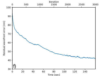
Residual wavefront error
