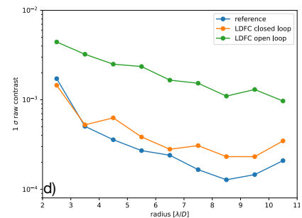
Raw contrast in dark hole
