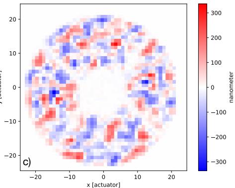
Residual wavefront error
