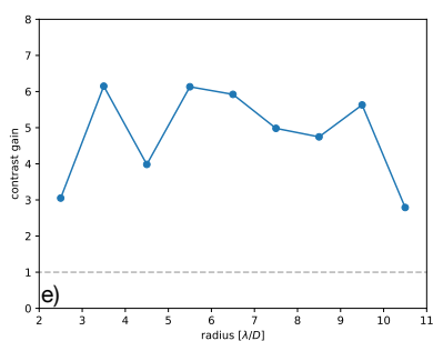
Raw contrast gain
