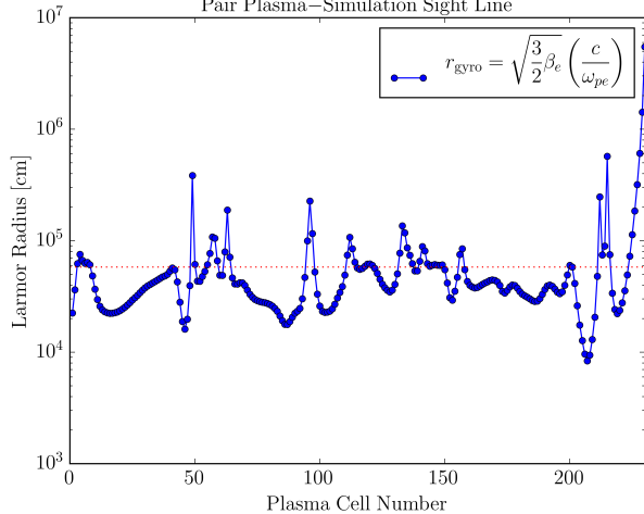
Pair Plasma—Simulation Sight Line
