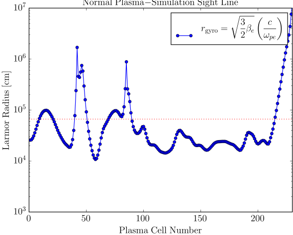
Normal Plasma—Simulation Sight Line
