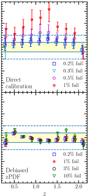
Misclassified lines
