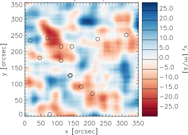
Vertical velocity at depth 25 Mm
