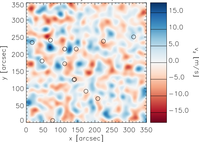
Vertical velocity at depth 0 Mm
