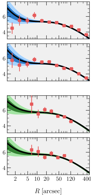
Model 6 (with IMBH)
