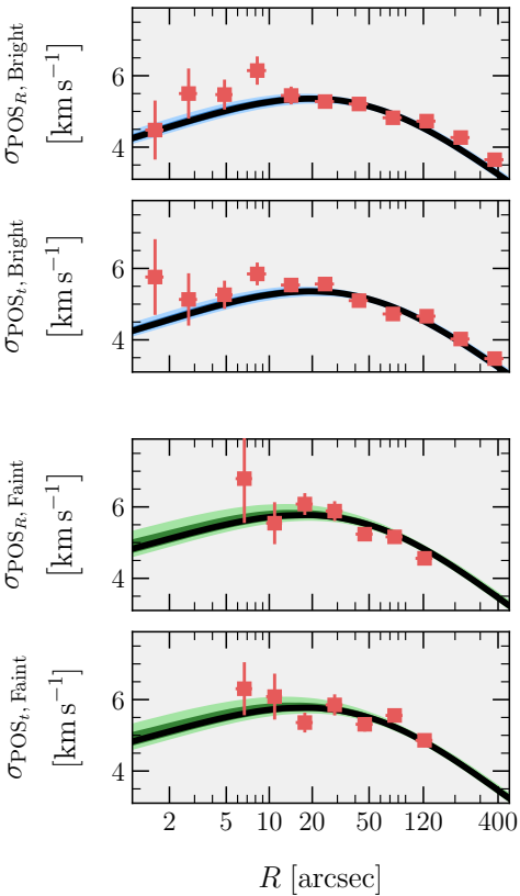
Model 8 (no dark component)
