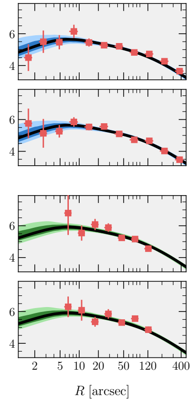
Model 14 (with CUO)
