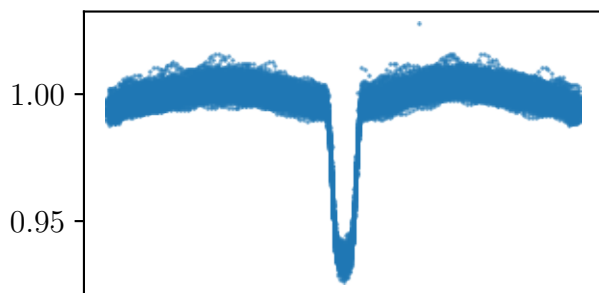
KIC2720354
