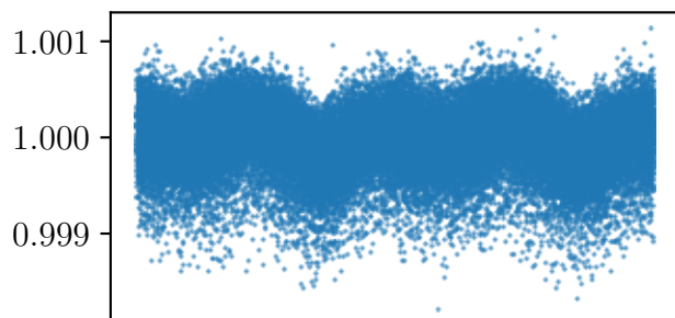
KIC4067110
