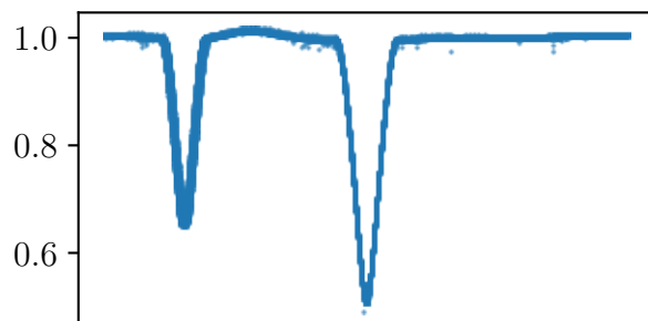
KIC4544587
