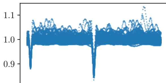
KIC3248332
