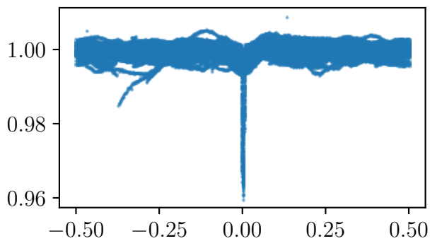
KIC10659313
