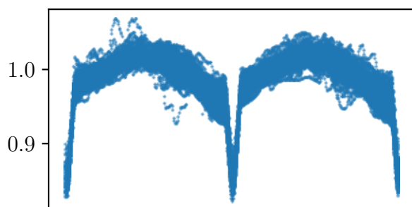
KIC5817566
