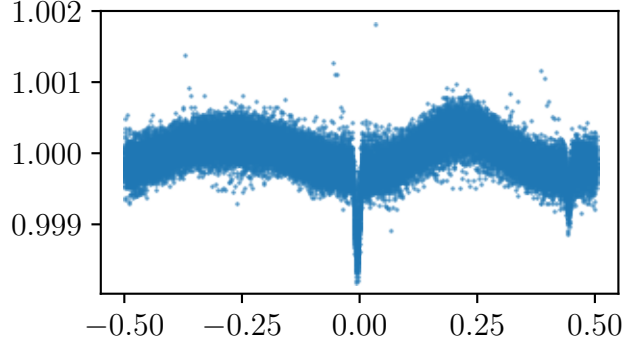
KIC12405950
