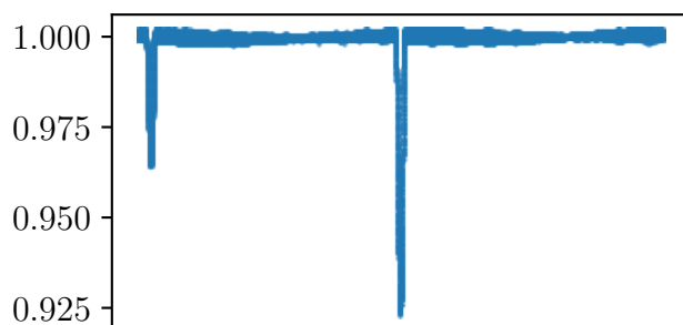
KIC8560861
