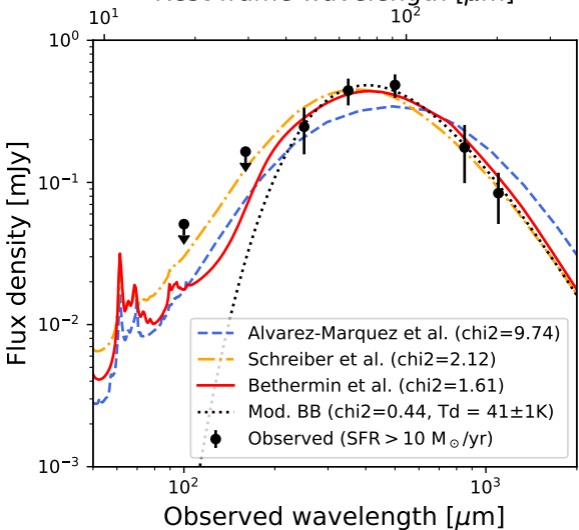
Stacked SED ( 4.0 < z < 5.0 and \text{SFR} > 10 M_{\odot}/\text{yr} ) Rest-frame wavelength [ \mu\text{m} ]
