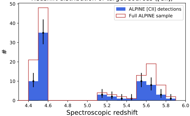
Redshift distribution of target sources ([CII])
