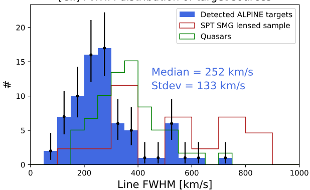
[CII] FWHM distribution of target sources
