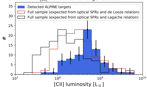
L_{[CII]} distribution of target sources
