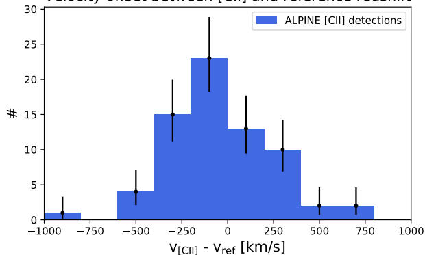
Velocity offset between [CII] and reference redshift
