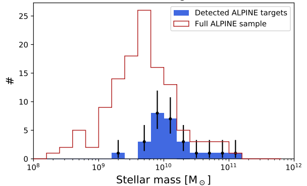
Stellar mass distribution of target sources (continuum)
