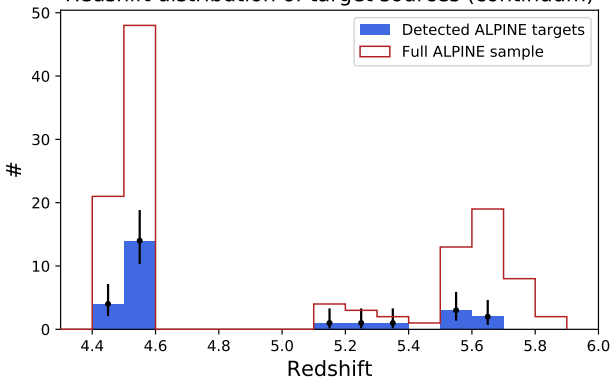
Redshift distribution of target sources (continuum)
