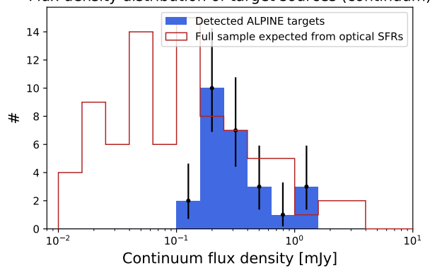
Flux density distribution of target sources (continuum)
