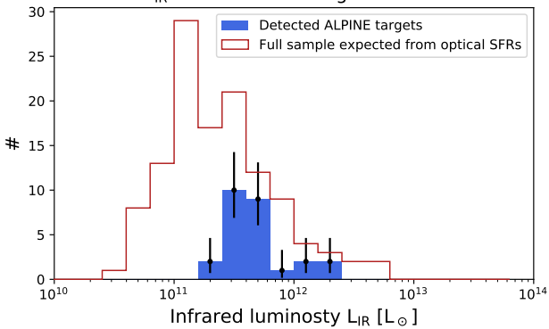
L_{\text{IR}} distribution of target sources
