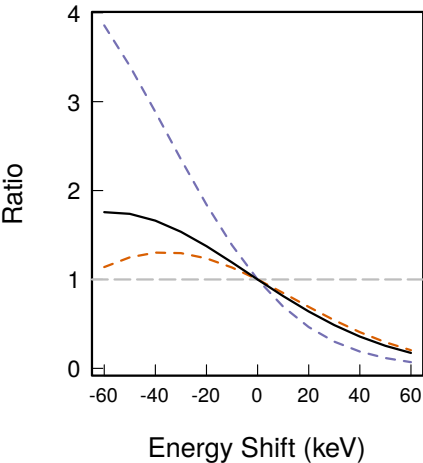
Correlated Energies
