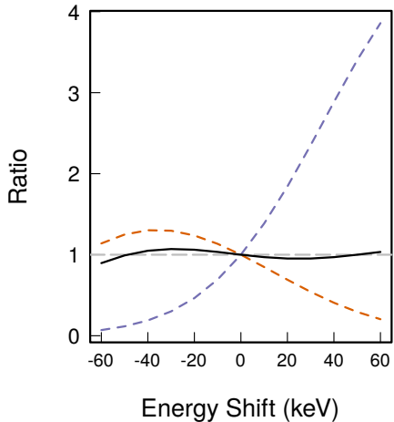
Anti-correlated Energies
