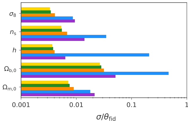
Model: \Lambda CDM - non-flat - pessimistic
