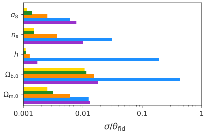
Model: \Lambda CDM - non-flat - optimistic
