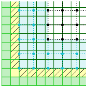
Lagrangian lattice and PM grid
