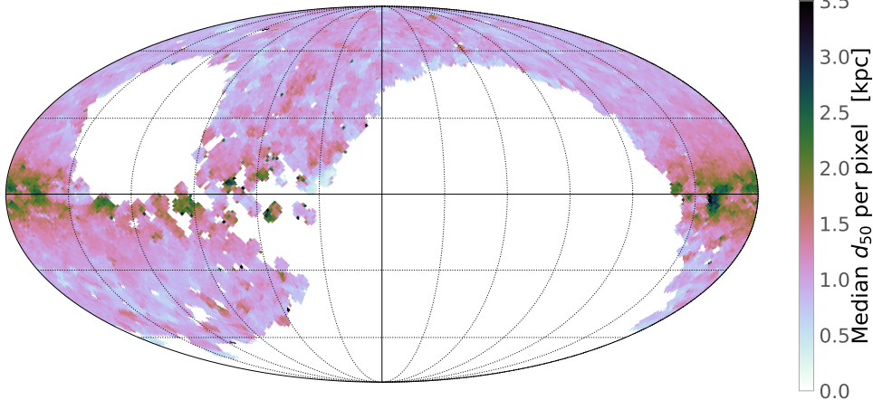
LAMOST DR5
