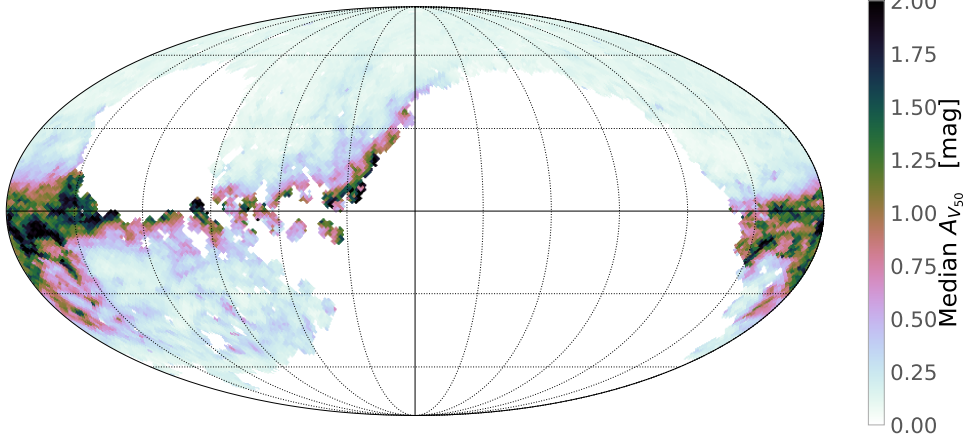
LAMOST DR5
