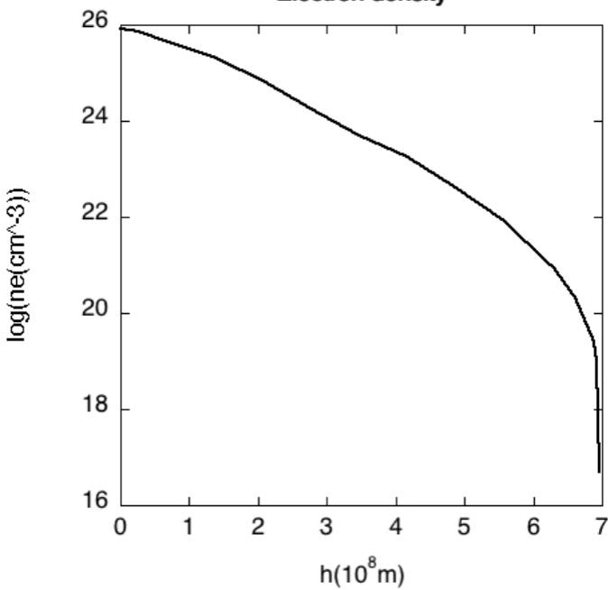
Electron density
