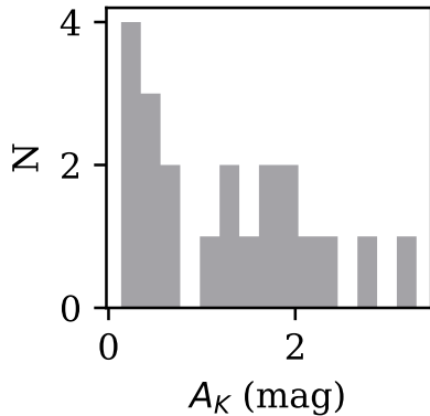
(b) G333.6-0.2
