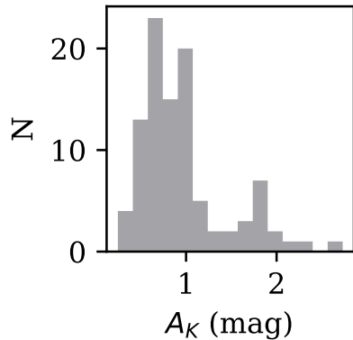
(c) NGC 6357
