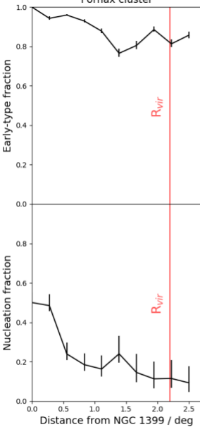
Fornax cluster
