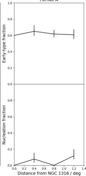
Fornax A
