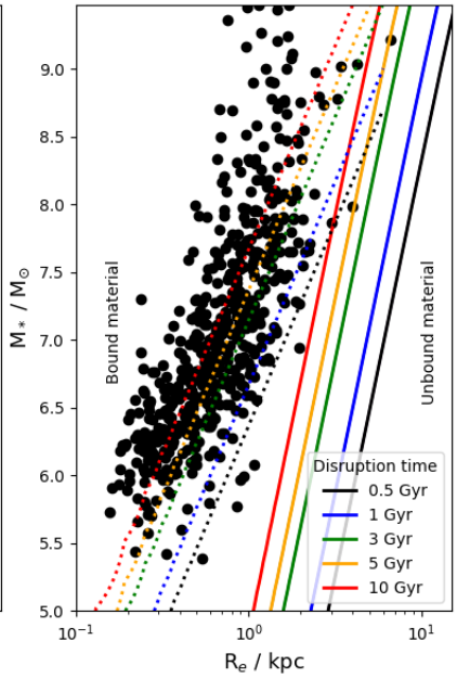
Galaxy-galaxy harassment
