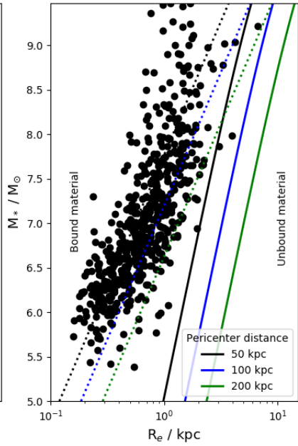
Tidal disruption
