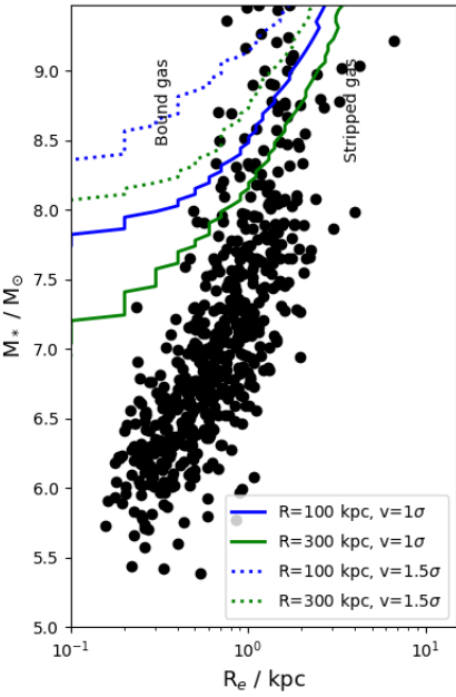
Ram Pressure Stripping
