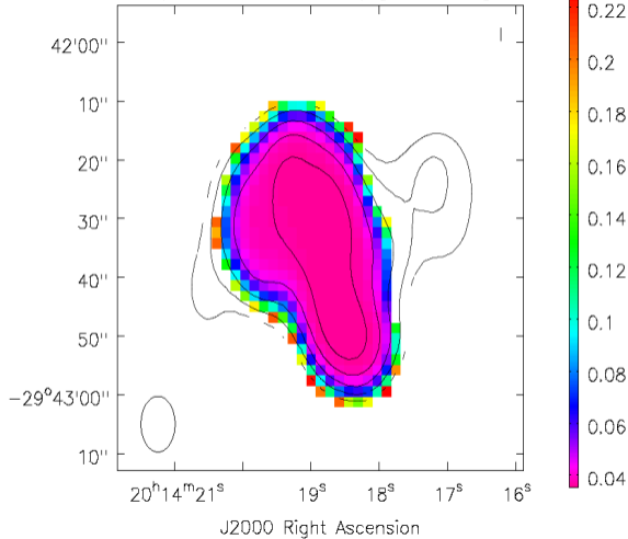
Spectral Index Error Map [1.7–9 GHz]
