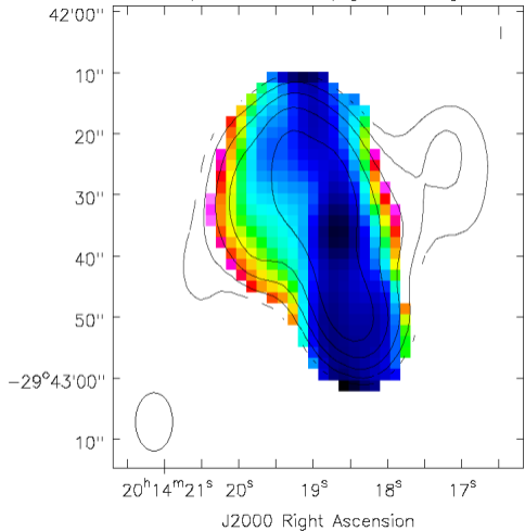
Spectral Index Map [1.7–9 GHz]
