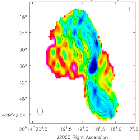
Spectral Index Map [5.5–9 GHz]
