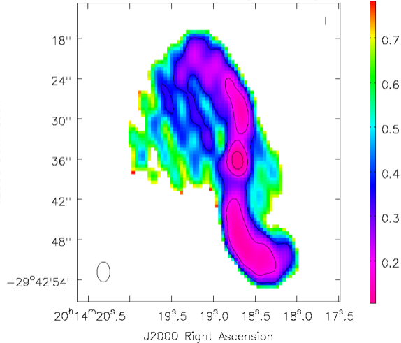
Spectral Index Error Map [5.5–9 GHz]
