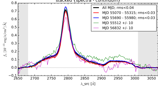
stacked {spectra - continuum} - {All MJD}
