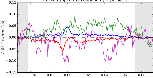
Mg II + Fe II model
