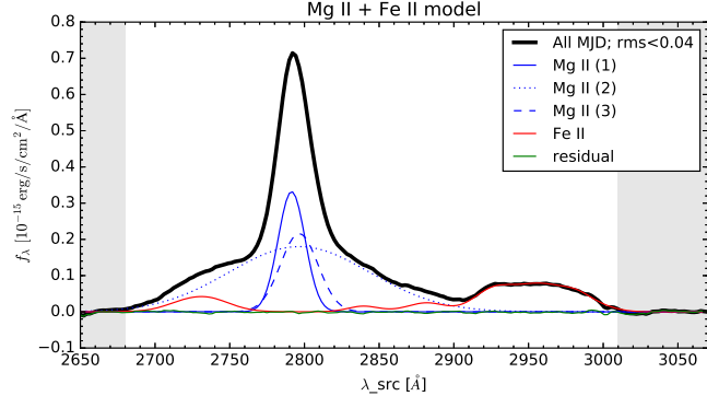
Mg II + Fe II model
