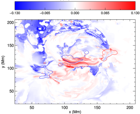
A_r^0 (FL) - A_r^0 (GP) - NLFF field
