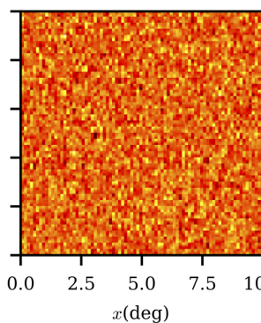
RCN-chip, \beta \delta \epsilon^*
