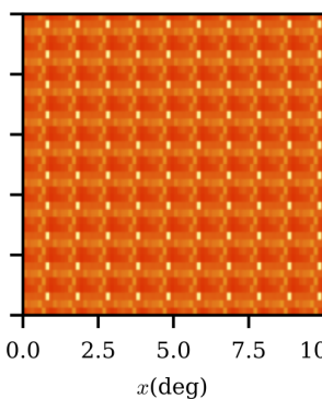
Regular Pattern, c(x, y)
