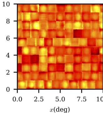
PSF leakage, \alpha \epsilon^*
