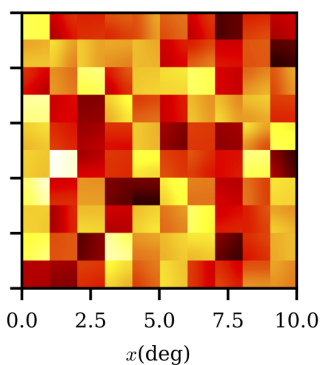
RCN-pointing, \beta \delta \epsilon^*
